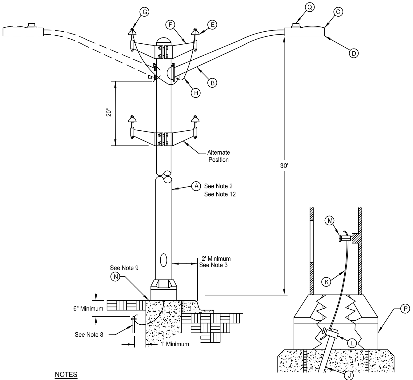
Grounding Detail
