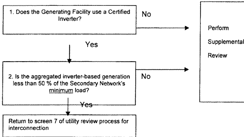
Figure 2: Utility Review Process for Interconnection to Network Systems
